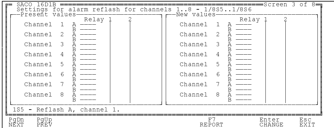
Fig. 2.4.4.C Configuration of the alarm reflash relays for channels 1 to 8 of the alarm module SACO 16D1B.
