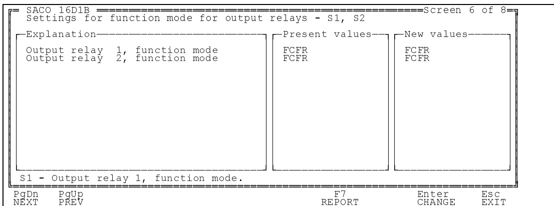
Fig. 2.4.4.F Settings for the operating mode of the output relays on the alarm module SACO 16D1B.
