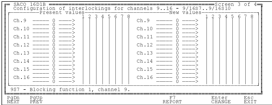
Fig. 2.4.3.C Configuration of interlocks for channels 9 to 16 of alarm module SACO 16D1B
