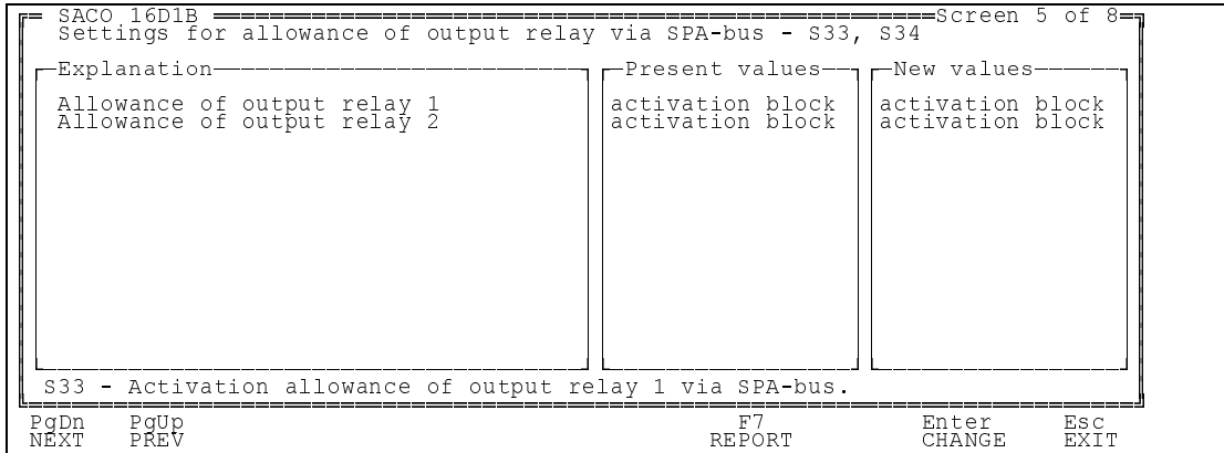
Fig. 2.4.4.E Settings for enabling output relays via the SPA bus on the alarm module SACO 16D1B.
