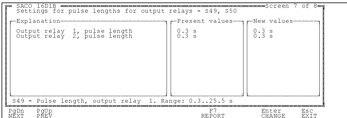
Fig. 2.4.4.G Setting the times output relays are energised (pulse length) on the alarm module SACO 16D1B.
