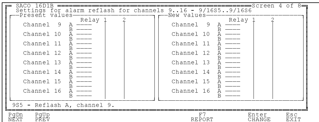
Fig. 2.4.4.D Configuration of the alarm reflash relays for channels 9 to 16 of the alarm module SACO 16D1B.
