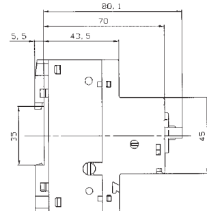
MS116 with aux. contact HKF 1 for front mounting
