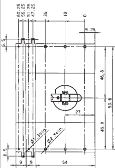
Drilling plan
