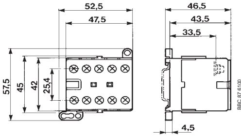
B 6(7)..., BC 6(7)..., K 6..., K C6..., for screw connection
